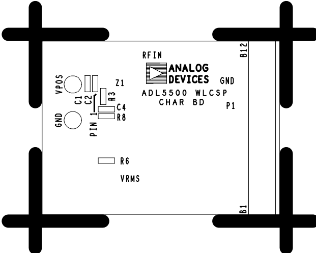
Figure 51. Silkscreen of Component Side (WLCSP)
