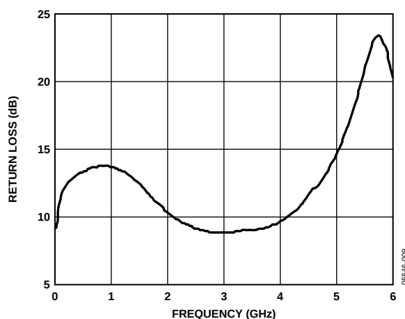
Figure 9. Return Loss vs. Frequency
