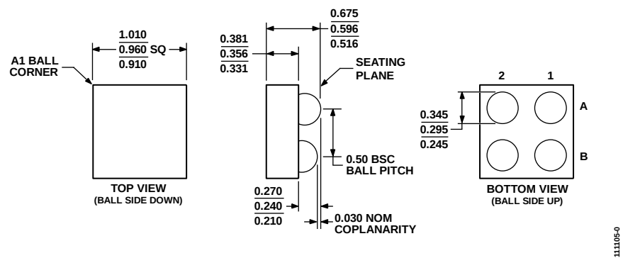
Figure 53. 4-Ball Wafer-Level Chip Scale Package [WLCSP] (CB-4) Dimensions shown in millimeters
