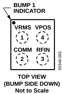
Figure 3. 4-Ball WLCSP Pin Configuration
