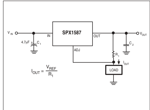
Figure 6. Current Source
