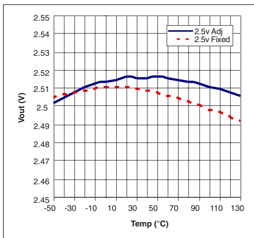
Figure 3. V_{IN}=4.0V , I_{OUT}=10mA
