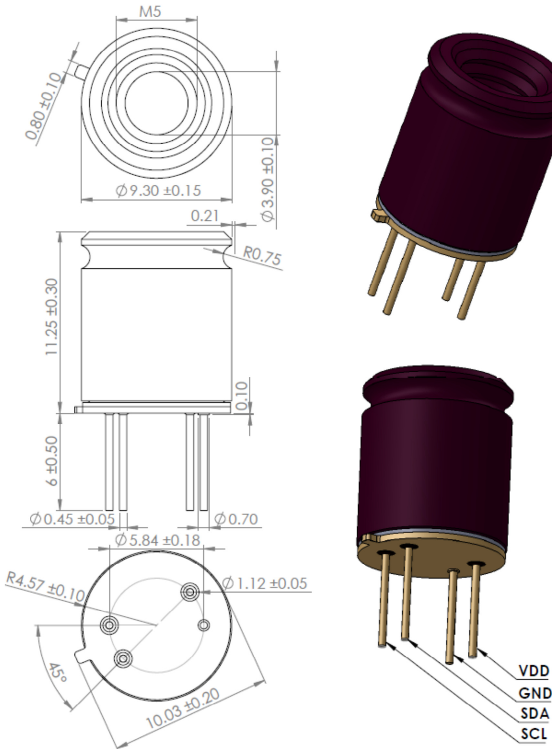
Figure 27 Mechanical drawing of 55° FOV device
