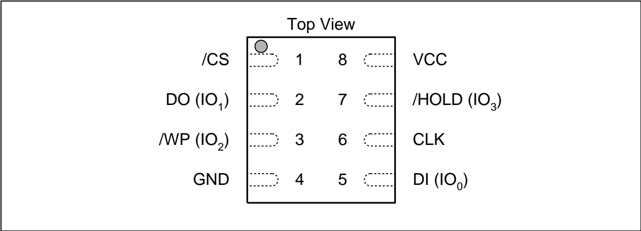
Figure 1b. W25Q80DV Pad Assignments, 8-pad WSON 6x5-mm
