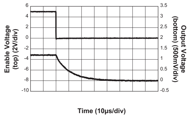
LDO Turn-Off Response ( V_{OUT} = 1.2V ; V_{IN} = 5V ; I_{OUT} = 400mA )
