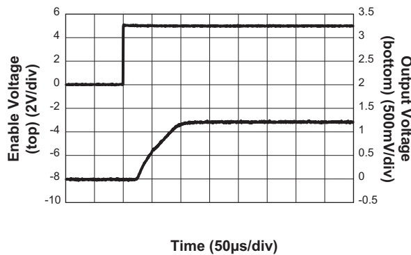
LDO Turn-On Response ( V_{OUT} = 1.2V ; V_{IN} = 5V ; I_{OUT} = 400mA )
