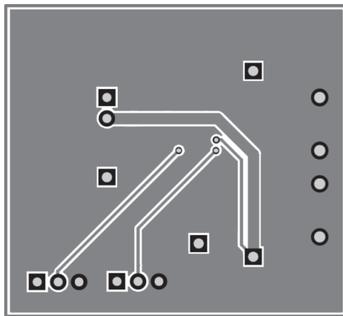
Figure 4: AAT2749-IUR Evaluation Board Bottom Layer.
