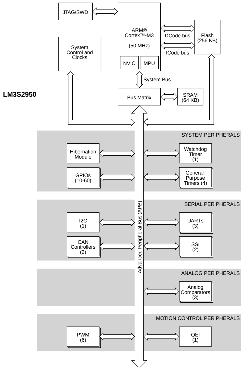
Figure 1-1. Stellaris® LM3S2950 Microcontroller High-Level Block Diagram
