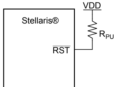
Figure 6-1. Basic RST Configuration
