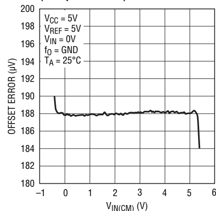
Offset Error vs V_{\text{IN(CM)}} (2x Speed Mode)
