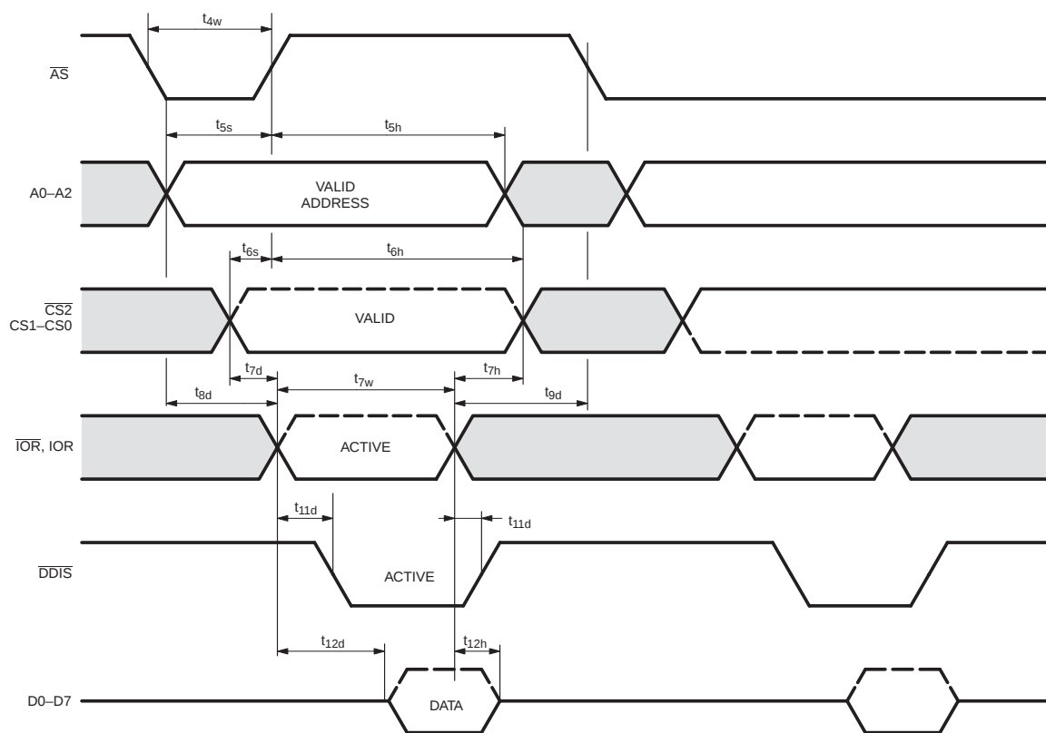
Fig 8. General read timing when using \overline{\text{AS}} signal.
