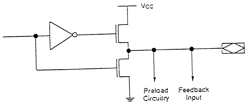
Typical Output
