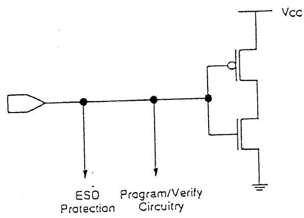
Typical Input
