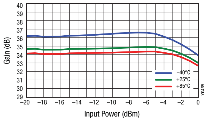
Figure 5. Gain vs Input Power over Temperature
