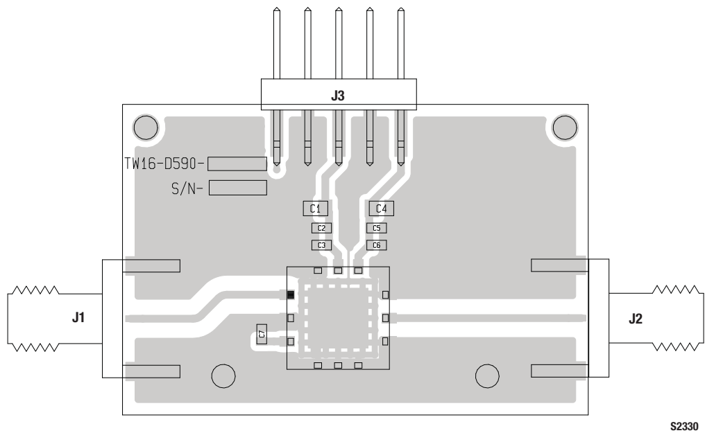
Figure 14. SKY65385-11 Evaluation Board Assembly Drawing
