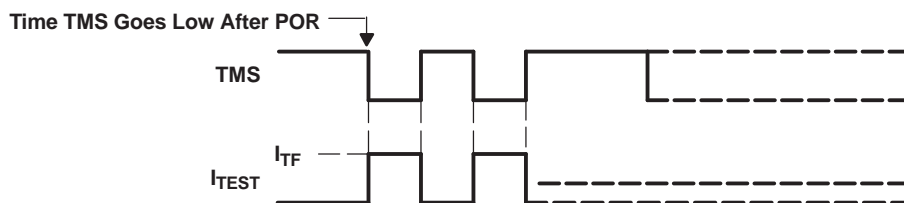
Figure 29. Fuse Check Mode Current, MSP430F22xx
