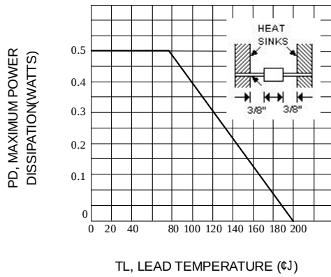
Fig. 1-STEADY STATE POWER DERATING
