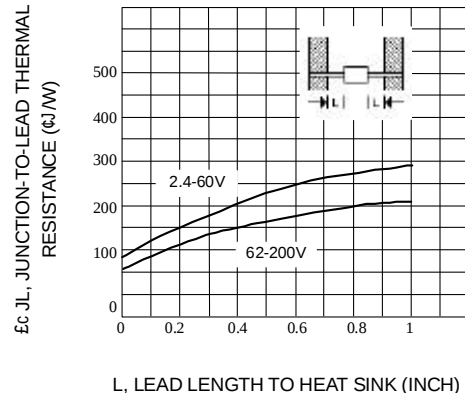
Fig. 2-TYPICAL THERMAL RESISTANCE
