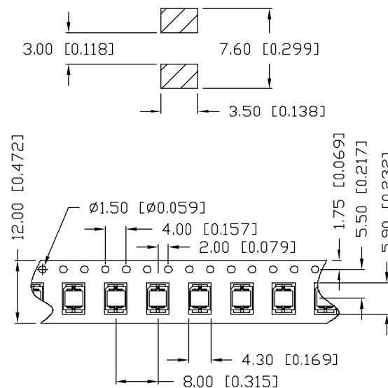
PAD LAYOUT
