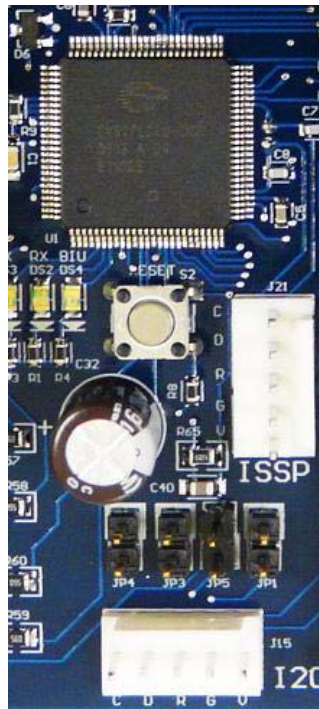
Figure 2-3. Development Section
