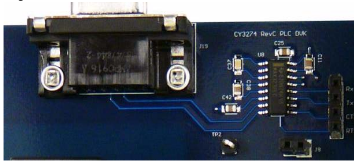
Figure 2-13. RS232- COM
