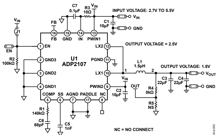
Figure 9. Evaluation Board Schematic of ADP2107-1.8-EVAL with V_{OUT} = 1.8 V
