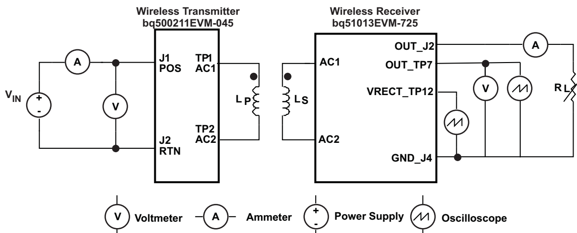
Figure 4. Equipment Setup
