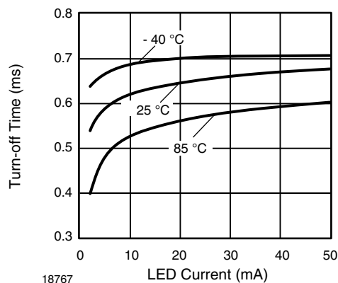
Fig. 20 - Turn-off Time vs. LED Current
