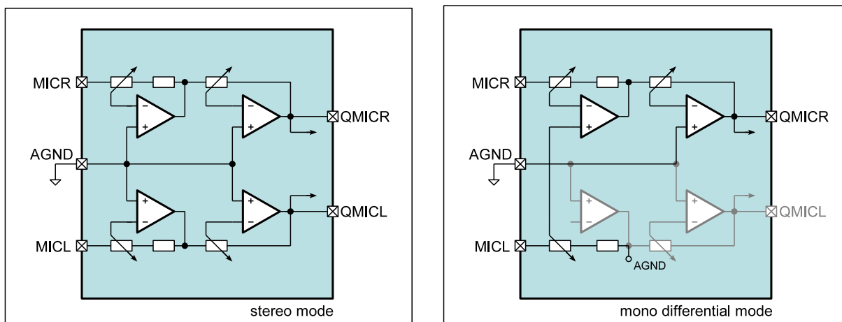
Figure 12. Microphone Input
