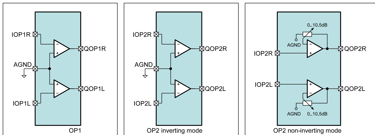
Figure 14. Operational Amplifiers
