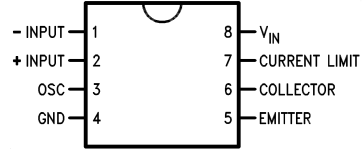
Dual-In-Line Package
