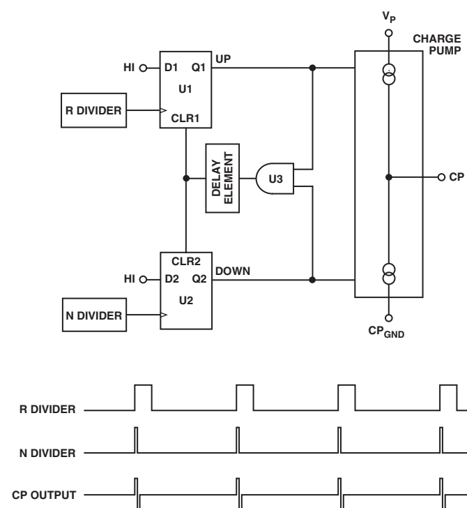
Figure 4. PFD Stage
