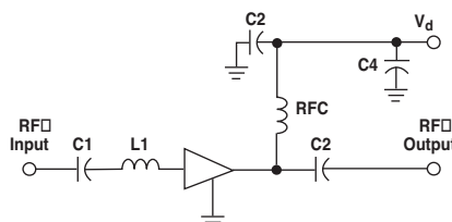
Figure 15. Schematic Diagram.
