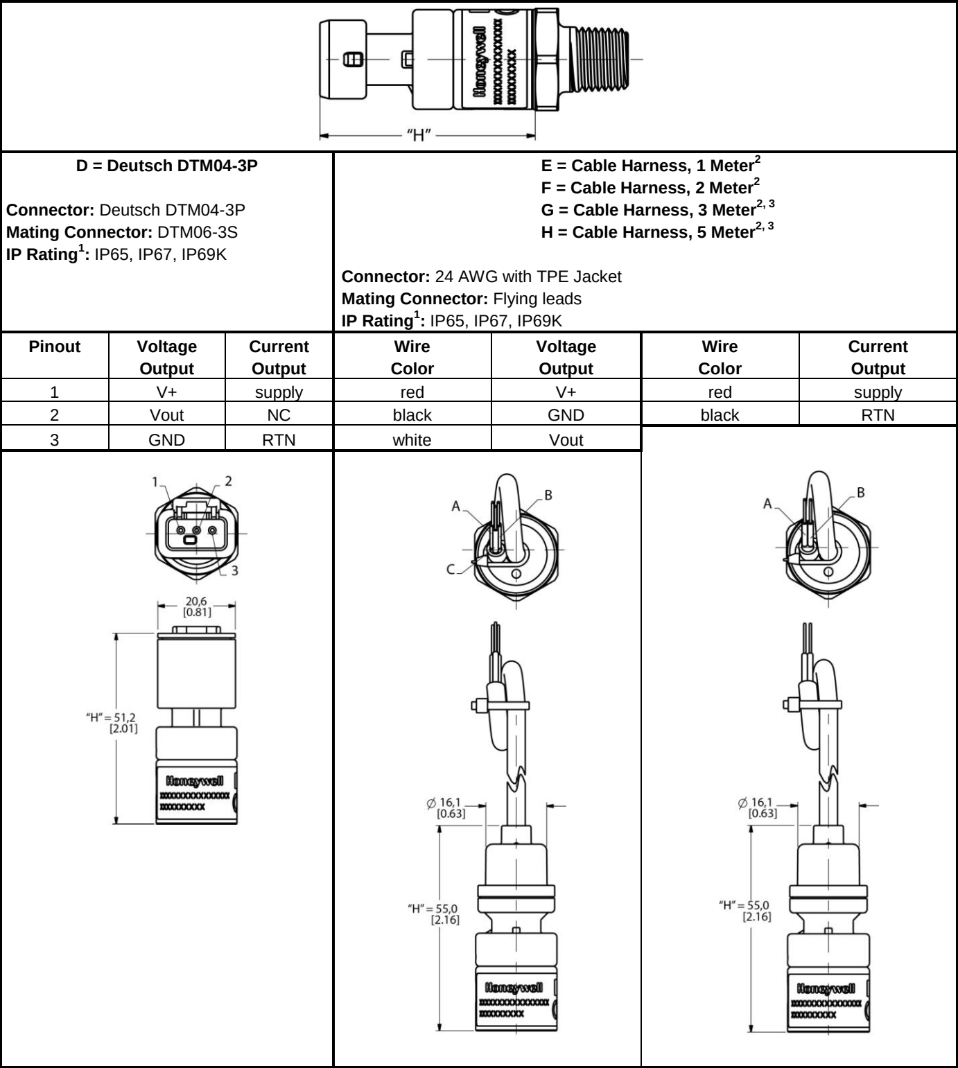
Figure 7. Connector Dimensions (For reference only: mm/[in], continued.)
