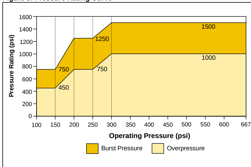
Figure 3. Pressure Rating Curve
