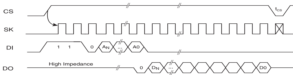
Figure 4-2. READ Timing
