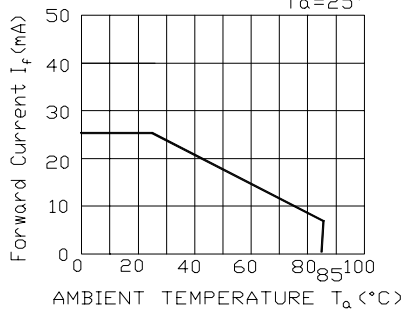
Forward Current Derating Curve T_a=25^\circ
