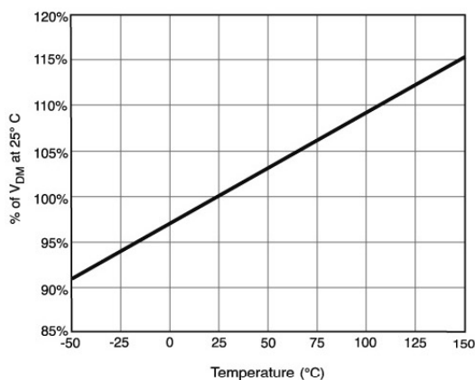
Figure SB3 - Off-state Voltage vs. Temperature
