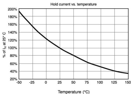
Figure SB5 - Hold Current vs. Temperature
