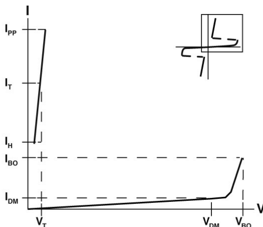
Figure SB1 - Voltage-Current Characteristics
