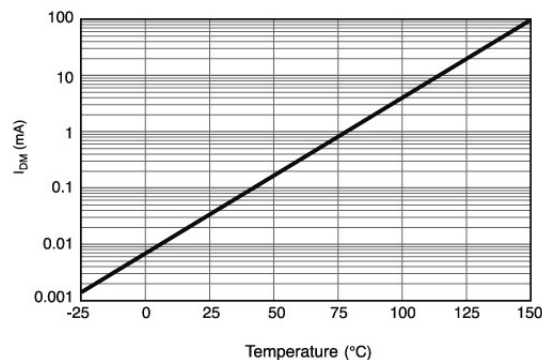
Figure SB6 - Off-state Current vs. Temperature
