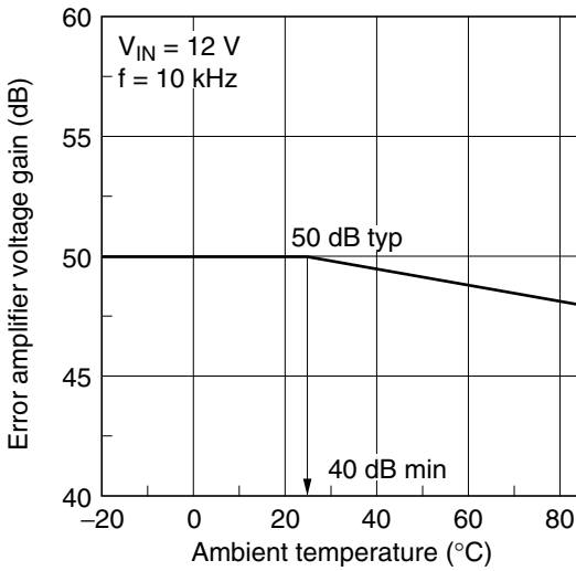
Error Amplifier Voltage Gain vs. Ambient Temperature
