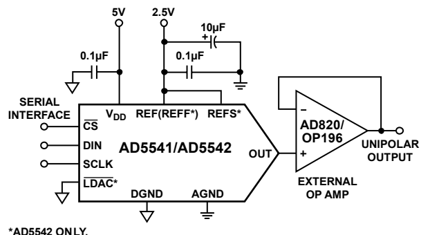
Figure 29. Unipolar Output
