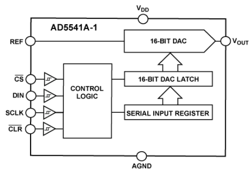
Figure 2. AD5541A-1
