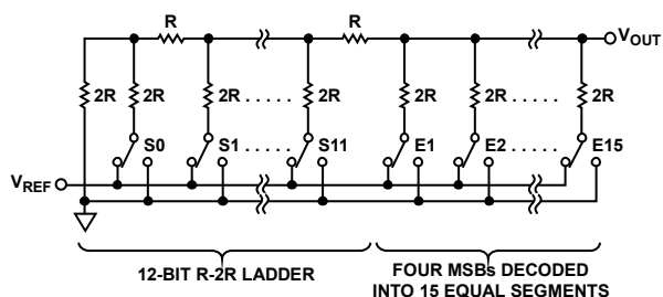
Figure 28. DAC Architecture
