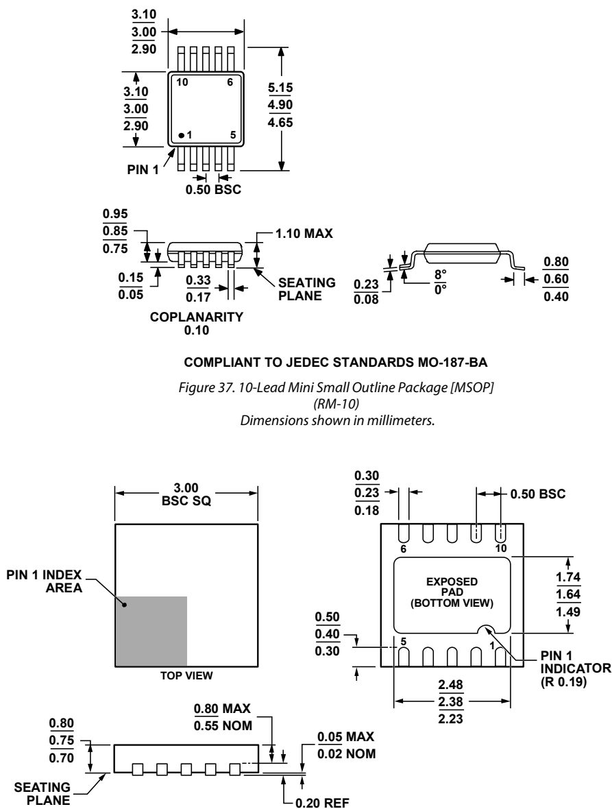
Figure 38. 10-Lead Lead Frame Chip Scale Package [LFCSP] (CP-10-9)
