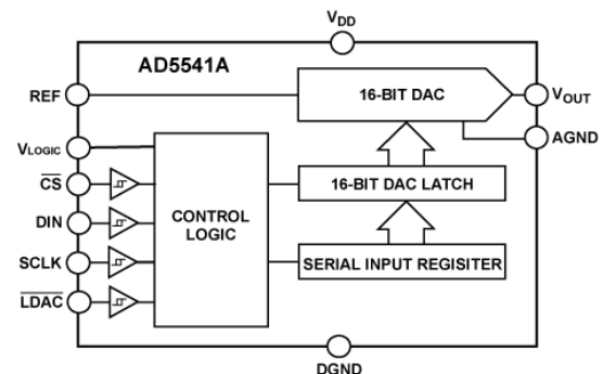
Figure 1. AD5541A
