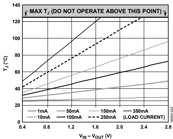
Figure 42. 0 mm 2 of PCB Copper, T_A = 25^{\circ}\text{C} , TSOT
