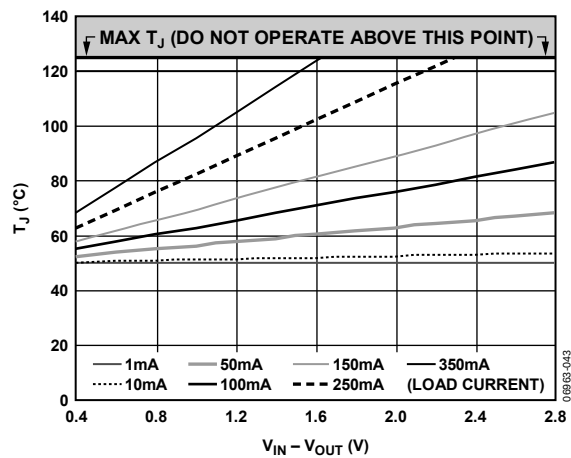
Figure 43. 500 mm 2 of PCB Copper, T_A = 50^{\circ}\text{C} , TSOT
