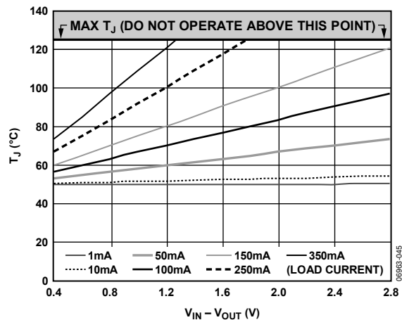
Figure 45. 0 mm 2 of PCB Copper, T_A = 50^{\circ}\text{C} , TSOT
