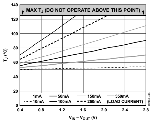
Figure 44. 100 mm 2 of PCB Copper, T_A = 50^{\circ}\text{C} , TSOT
