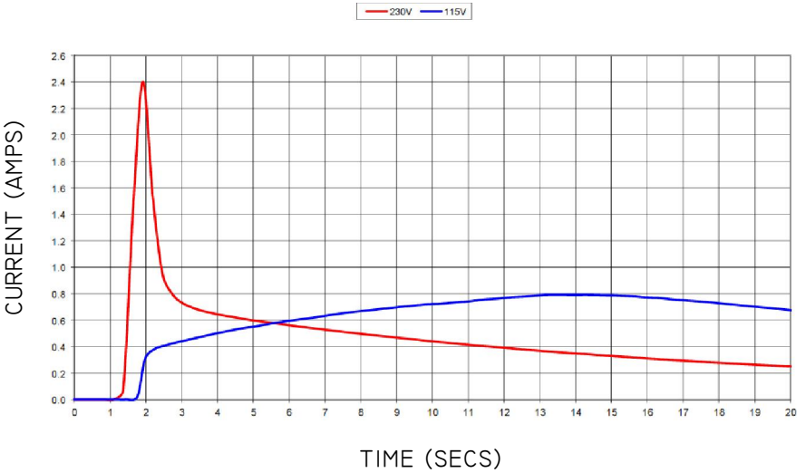
TYPICAL INRUSH GRAPH
