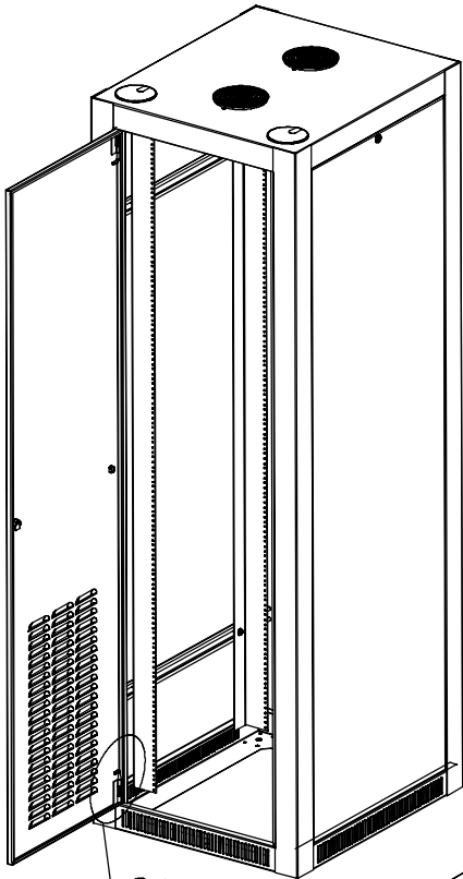
Hinge Pin Removal
