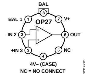
Figure 1. TO-99 (J-Suffix)
