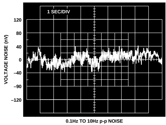
Figure 33. Low-Frequency Noise
