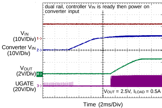
Power Sequence
