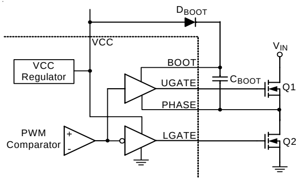
Figure 2. Gate Driver and Bootstrap Circuit
