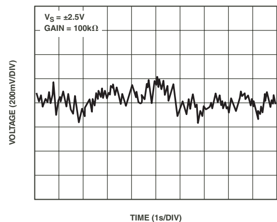
TPC 15. Input Voltage Noise
