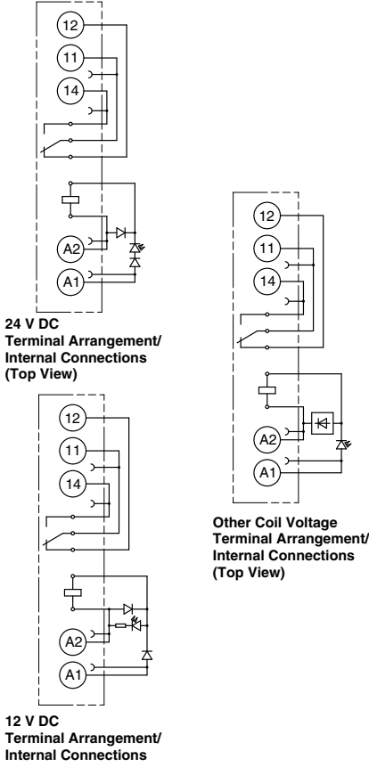
Input circuit
