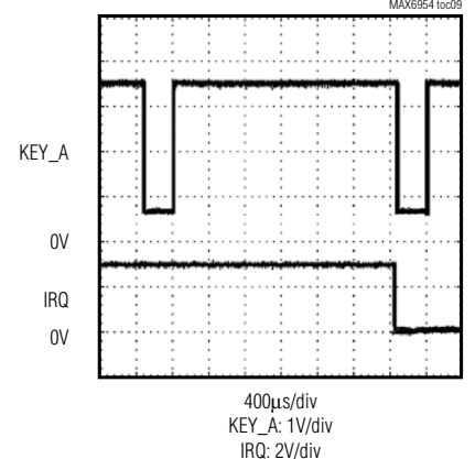
KEY-SCAN OPERATION (KEY_A AND IRQ)
