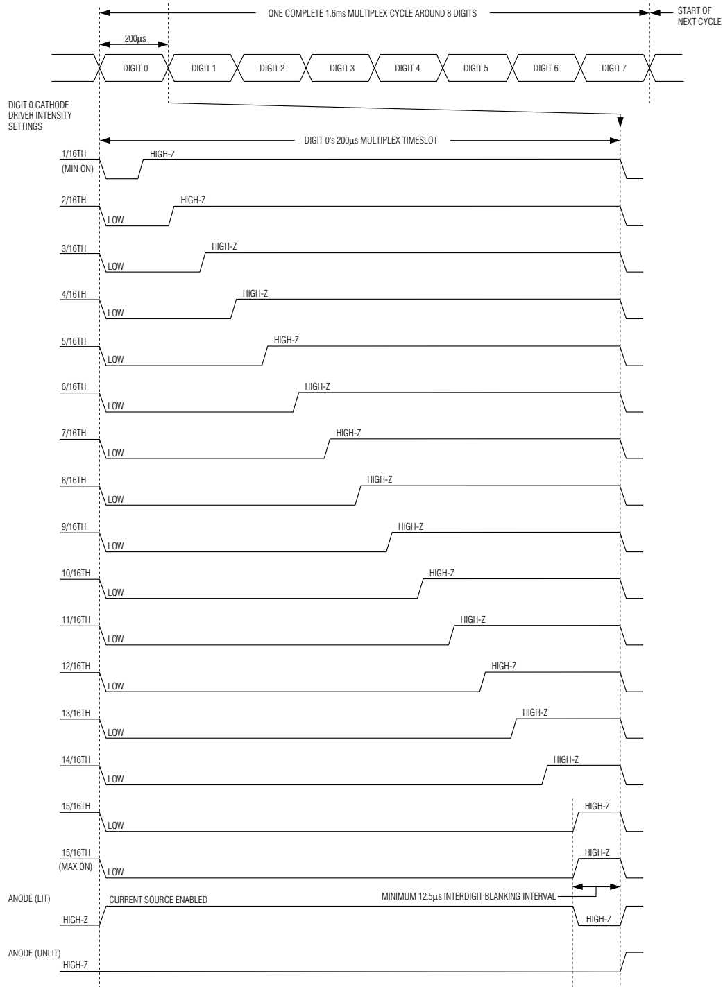
Figure 10. Multiplex Timing Diagram (OSC = 4MHz)
