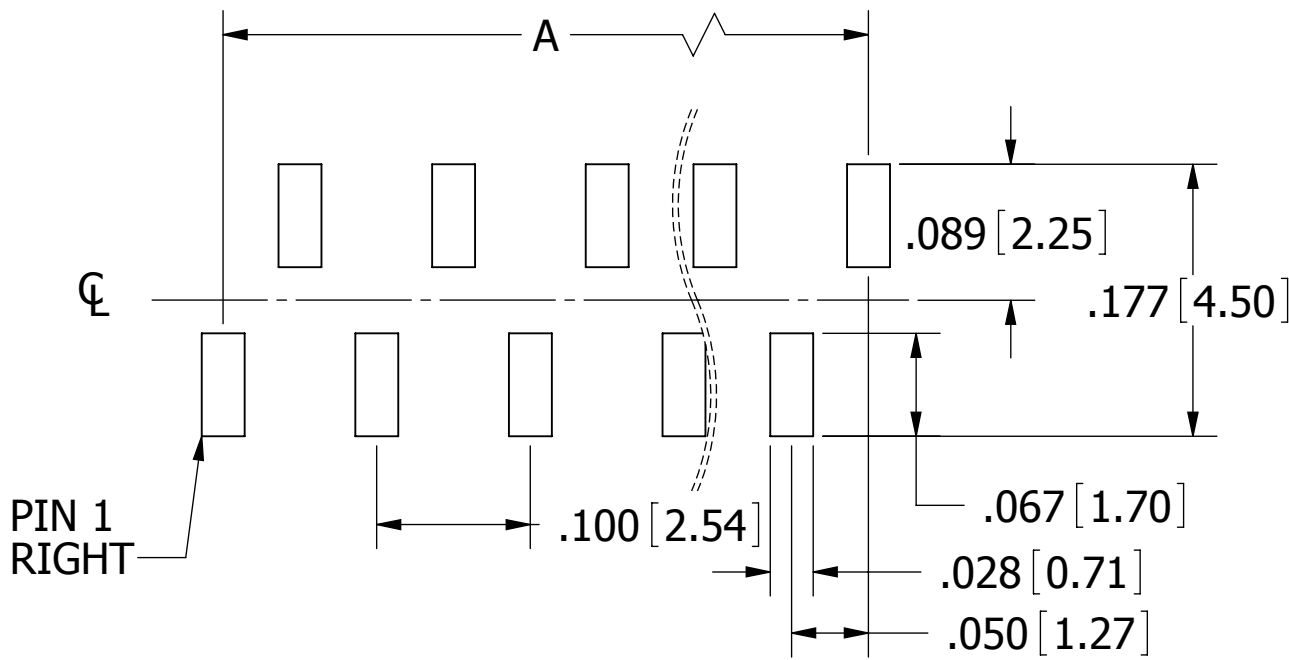
RECOMMENDED PCB SMD LAYOUT GRP B _ 1 VWTD-RC
