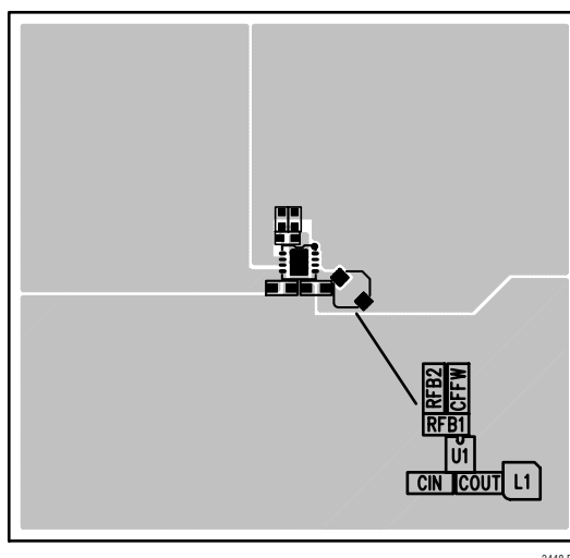
Figure 8. LTC3448 Layout
