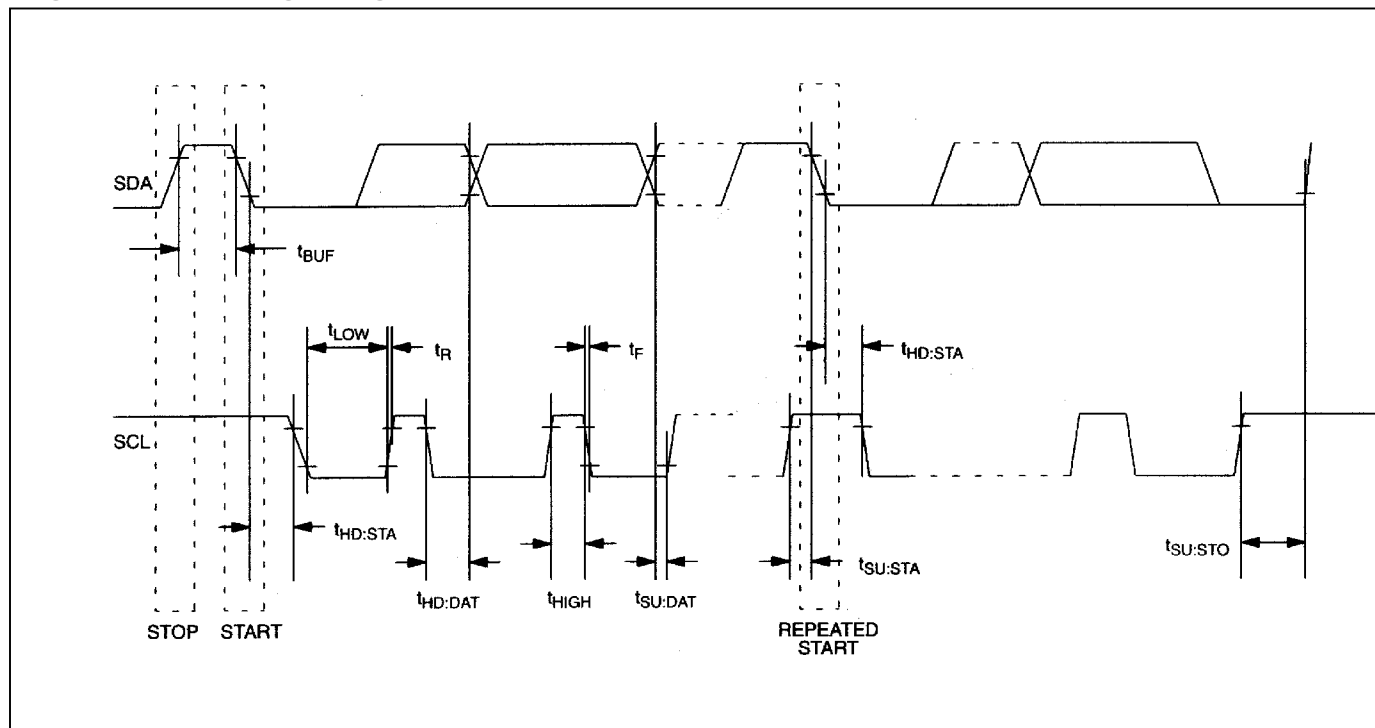
Figure 1. Timing Diagram
