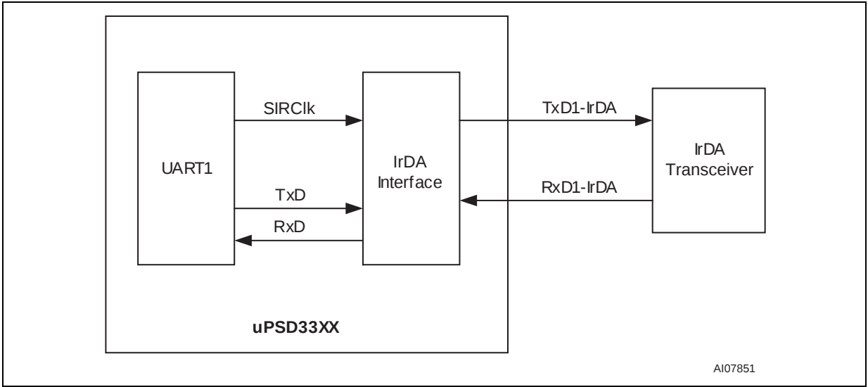
Figure 36. IrDA Interface
