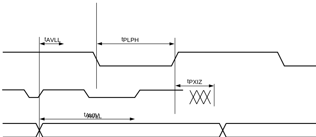
Figure 88. External \overline{\text{PSEN}} /READ Cycle (80-pin Device Only)
