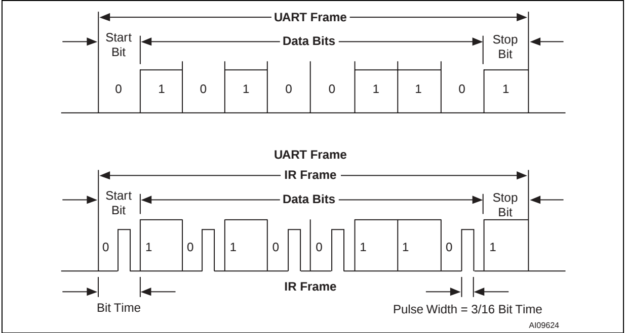
Figure 37. Pulse Shaping by the IrDA Interface
