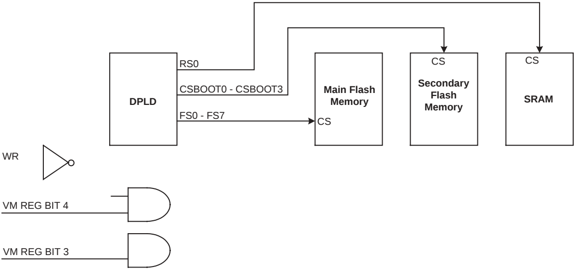
Figure 59. VM Register Control of Memories
