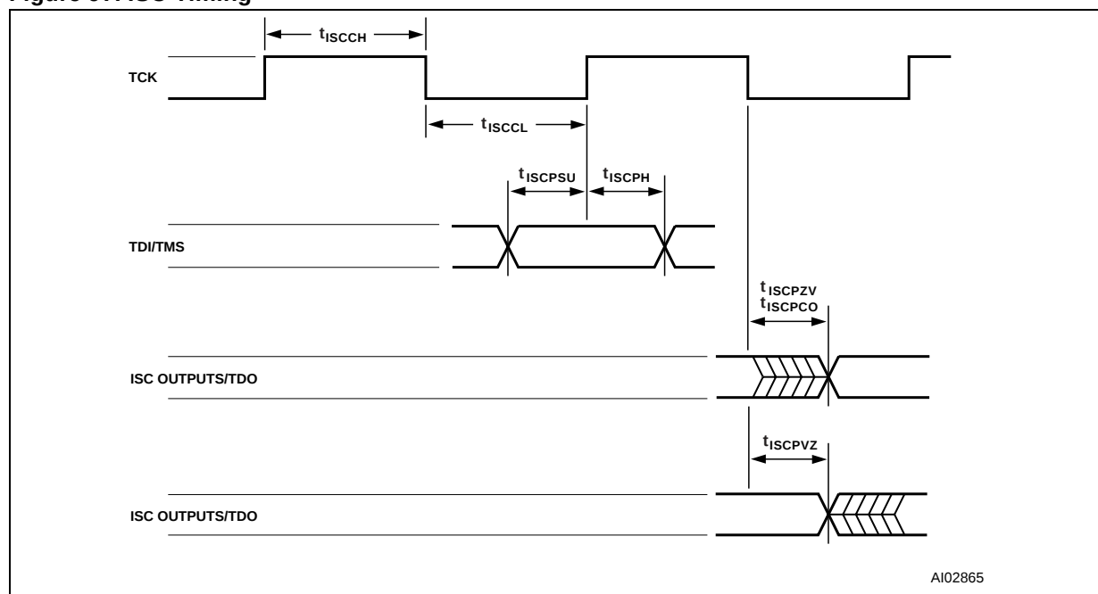
Figure 97. ISC Timing
