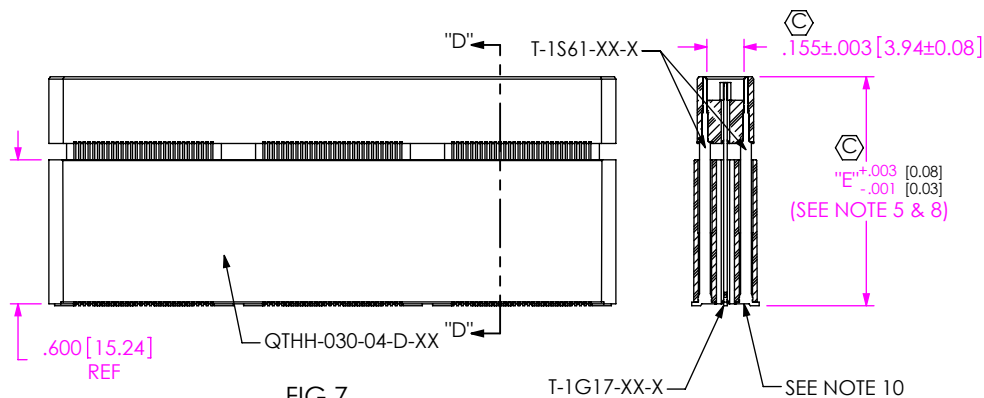
FIG 7 (QTH-090-07-X-D SHOWN) (SAME AS FIG 5, EXCEPT AS SHOWN)
