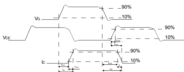
Figure 19. Switching waveform
