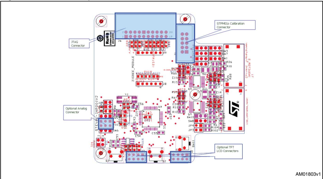
Figure 5. Connector position
