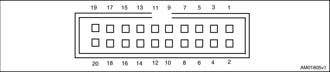
Figure 7. Debug connector
