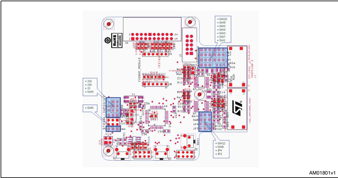
Figure 3. Jumper placement
