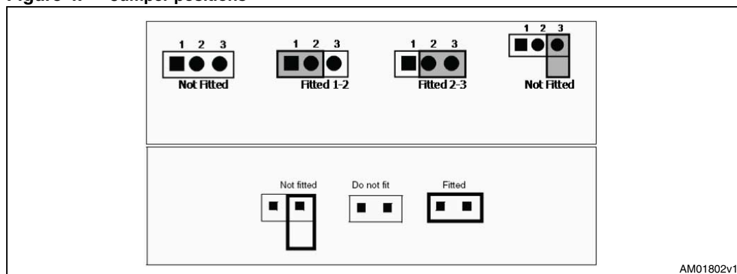
Figure 4. Jumper positions
