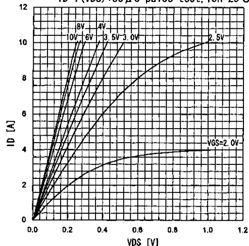
出力特性 Typical output characteristics
