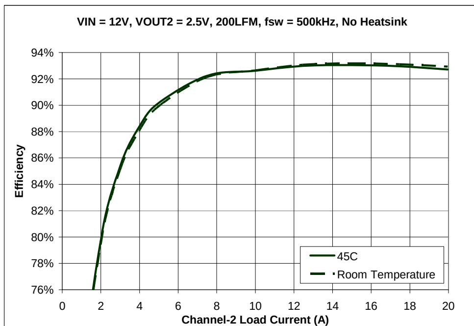
Fig. 23 Channel-2 Efficiency
