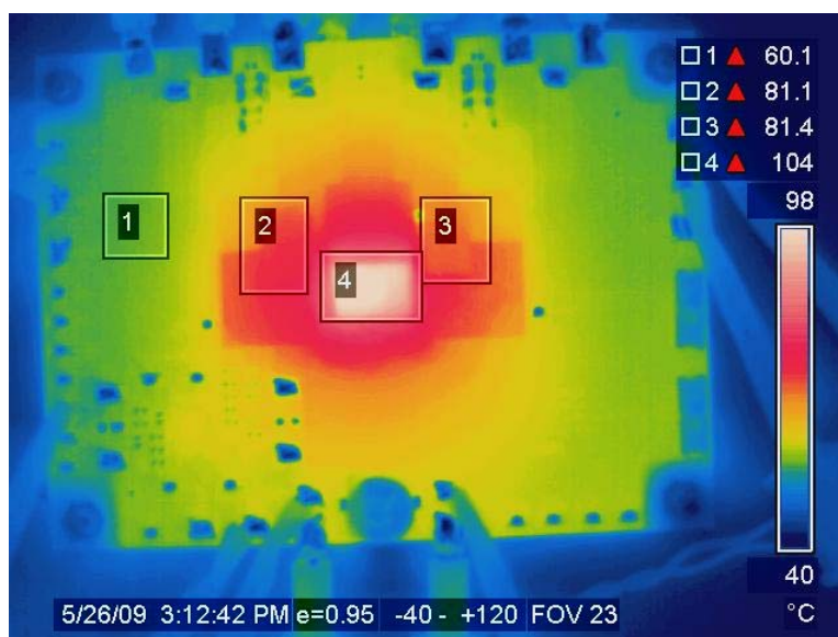
Fig. 24 Thermal Image: I_{out} = 20A per channel, V_{IN} = 12V , V_{OUT1} = 1.5V , V_{OUT2} = 2.5V , T_A = 45^{\circ}C , f_{sw} = 500kHz , 200LFM, No Heatsink, Maximum Temperature = 104^{\circ}C
