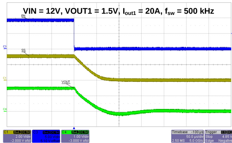
Fig. 6 Channel-1 Power Down Sequence (C3: EN, C1: SS1, C4: VOUT1)
