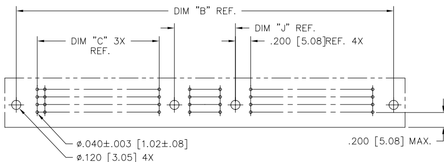
SECTION U-U
