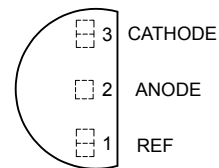
Figure 2. Pin Configuration of AZ431-B (Top View)
