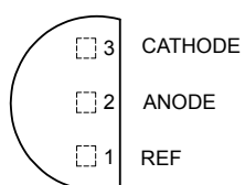
Figure 2. Pin Configuration of AZ431-B (Top View)
