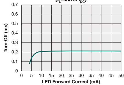
Typical Turn-Off vs. LED Forward Current ( I_L=50\text{mA}_{DC} )
