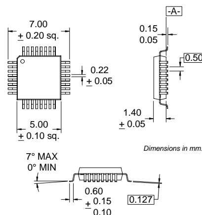
Package Style: LQFP-32_5x5
