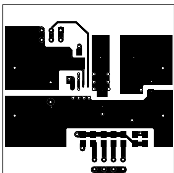
Figure 6c. Top-Side Copper
