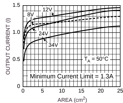
Figure 3. Output Current vs. Ground Plane Area
