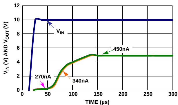
FIGURE 53. TURN-ON TIME
