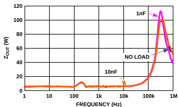
FIGURE 54. Z_{OUT} vs FREQUENCY
