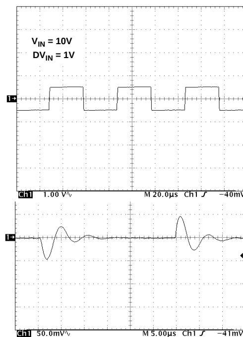
FIGURE 52. LINE TRANSIENT RESPONSE, 0.001 \mu F LOAD CAPACITANCE
