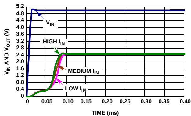
FIGURE 25. TURN-ON TIME
