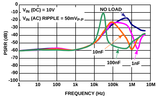
FIGURE 50. PSRR AT DIFFERENT CAPACITIVE LOADS
